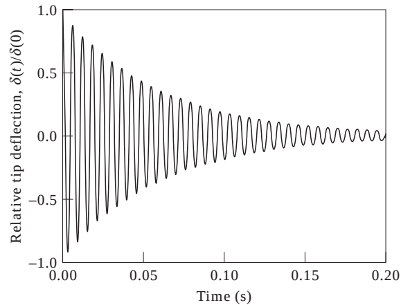
Figure 7. The effect of negative velocity gain on the cantilever composite beam subjected to first mode vibration (five pairs of S/As). Gain = -1.0\text{E}4 V/A.
