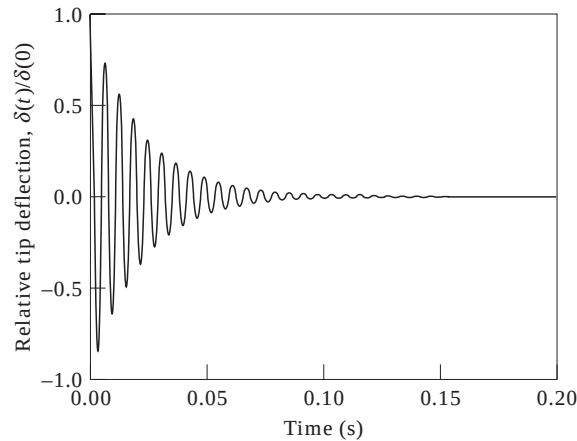
Figure 9. The effect of negative velocity gain on the cantilever composite beam subjected to first mode vibration (five pairs of S/As). Gain = -5.0 \times 10^4 V/A.
