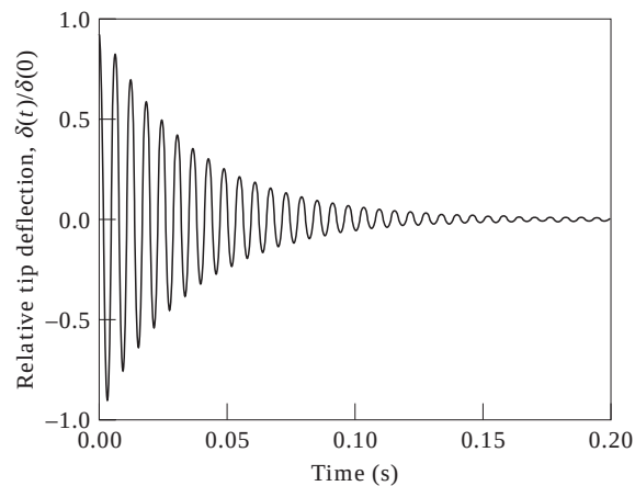
Figure 8. The effect of negative velocity gain on the cantilever composite beam subjected to first mode vibration (five pairs of S/As). Gain = -2.5\text{E}4 V/A.
