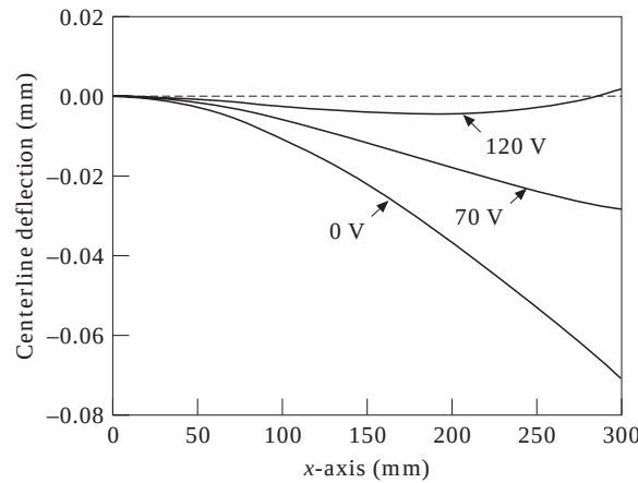
Figure 2. The centerline deflection of the cantilever composite beam with five pairs of actuators evenly distributed.
