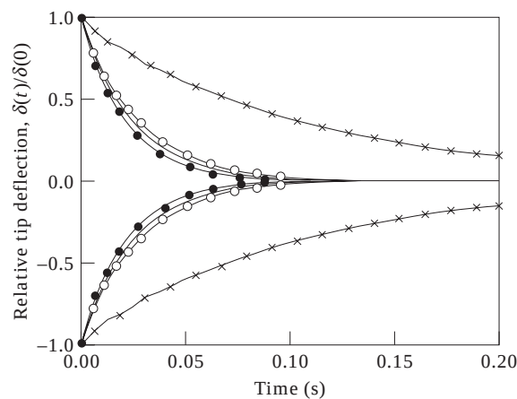
Figure 10. Decay envelopes of the tip displacement \delta(t) for the cantilever composite beam with different pairs of S/As (Gain = -5.0 \times 10^4 V/A). —x—, Uncontrolled; —●—, five pairs; —, two pairs; —○—, one pair.
